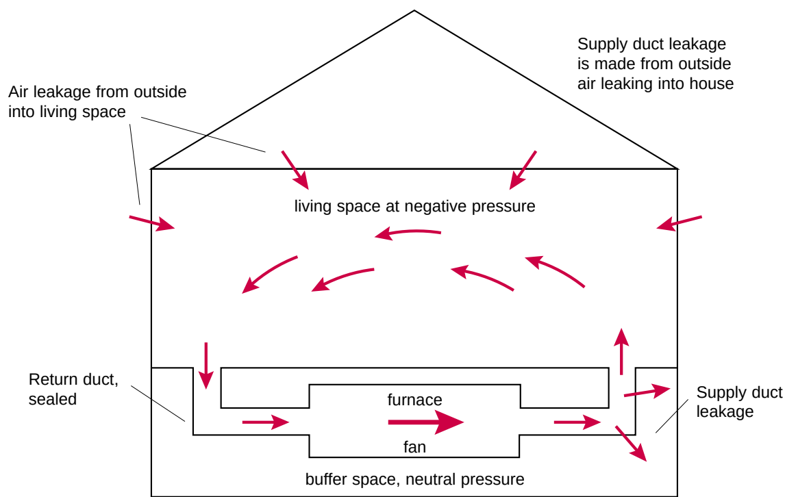
Figure 3. Duct Systems With Supply Side Leaks
