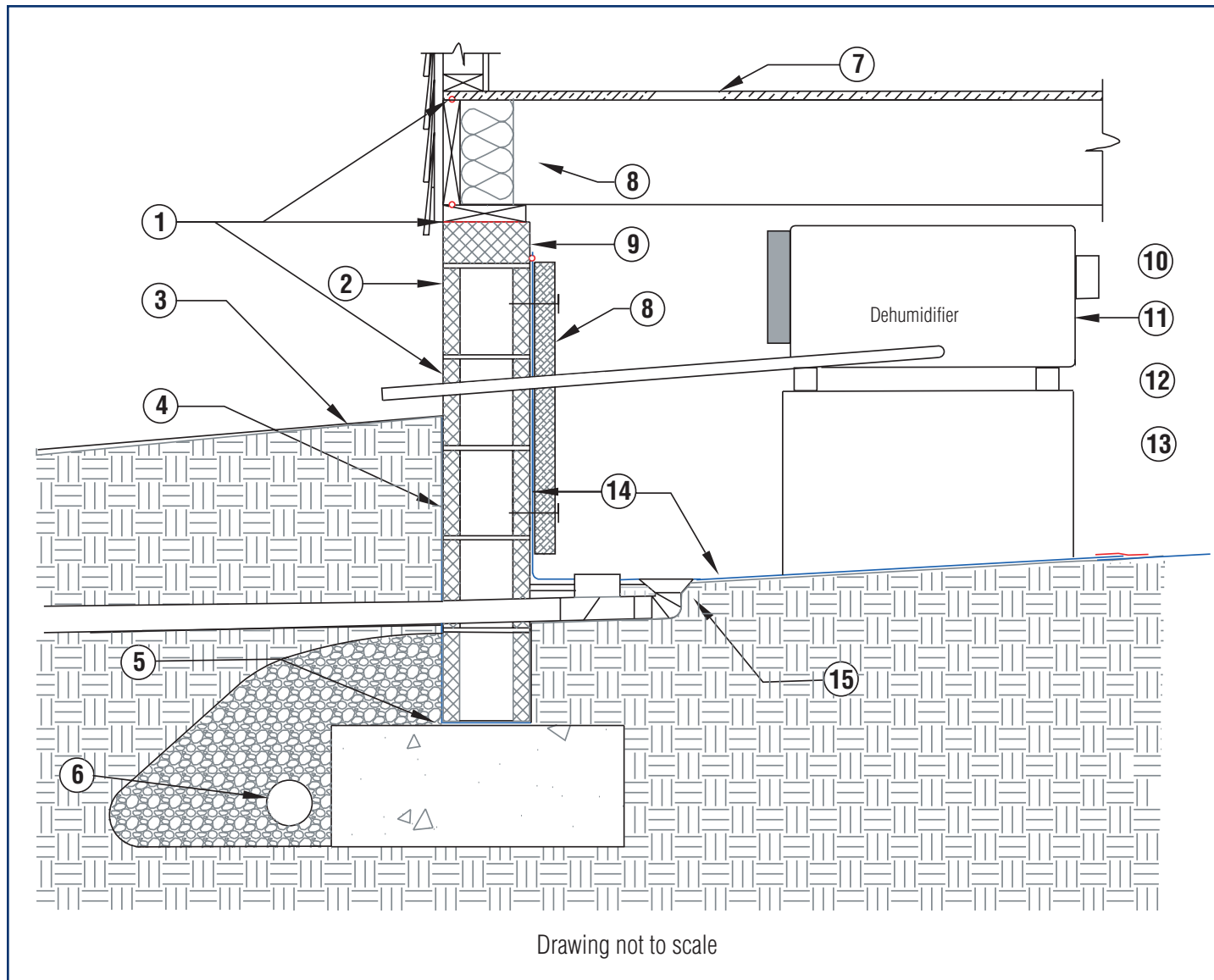
Advanced Energy Sample Design: A Closed Crawl Space With Dehumidifier and Wall Insulation
